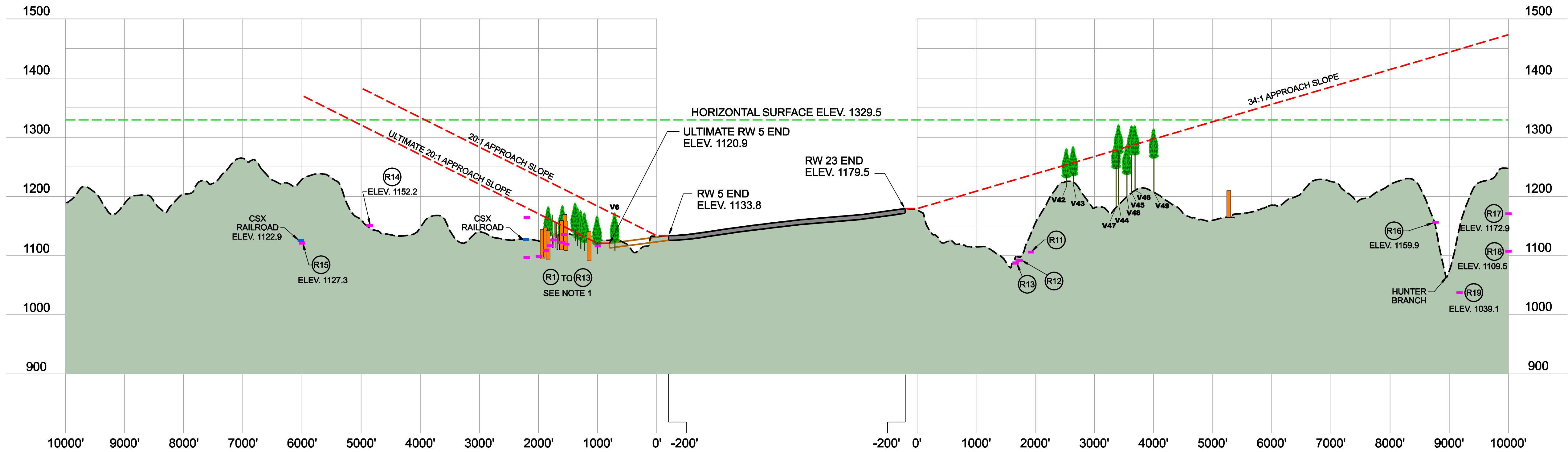
PROFILE VIEW SCALE: 1"=1000' HORIZONTAL 1"=100' VERTICAL
